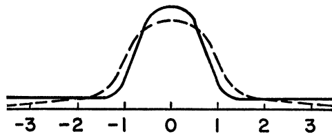
Standardized Variable
